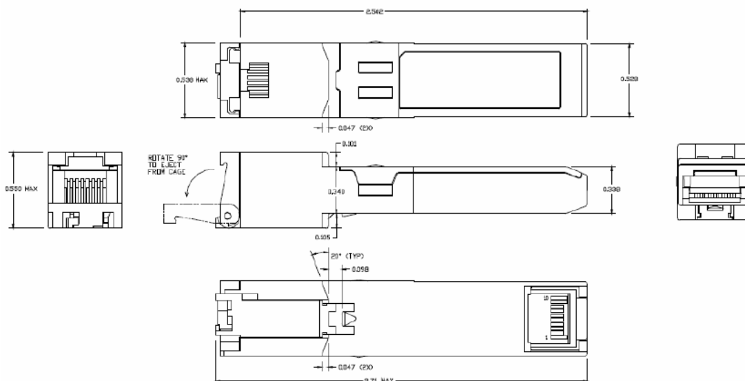
Figure 2. SFP GE T mechanical dimensions
